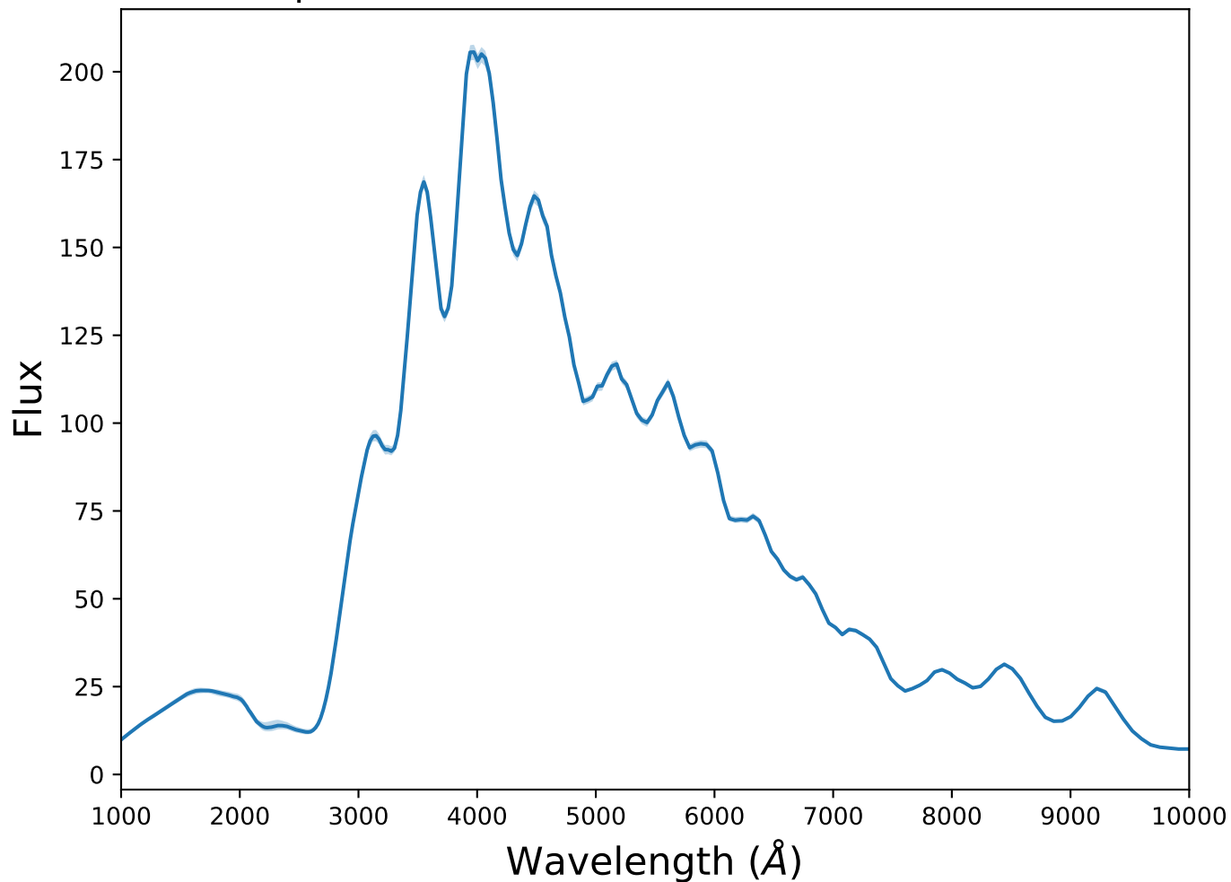
Spectrum 5 for transient SNIa at z=1.01
